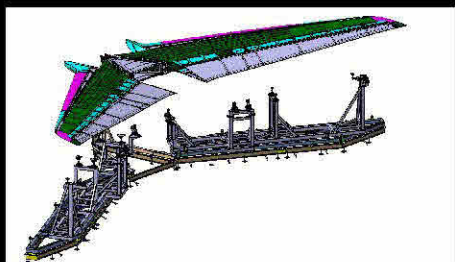
TAIL STABILYSER
